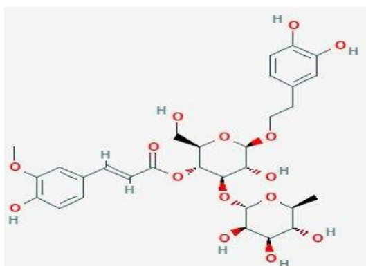
Leucosceptoside A
