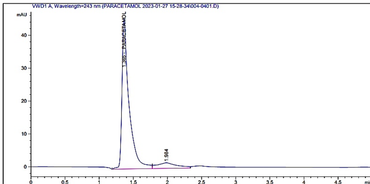
Figure 1b: Chromatographic peak for paracetamol injection sample (Vinco®) (15 µg/mL) at a retention time of 1.365 minute
